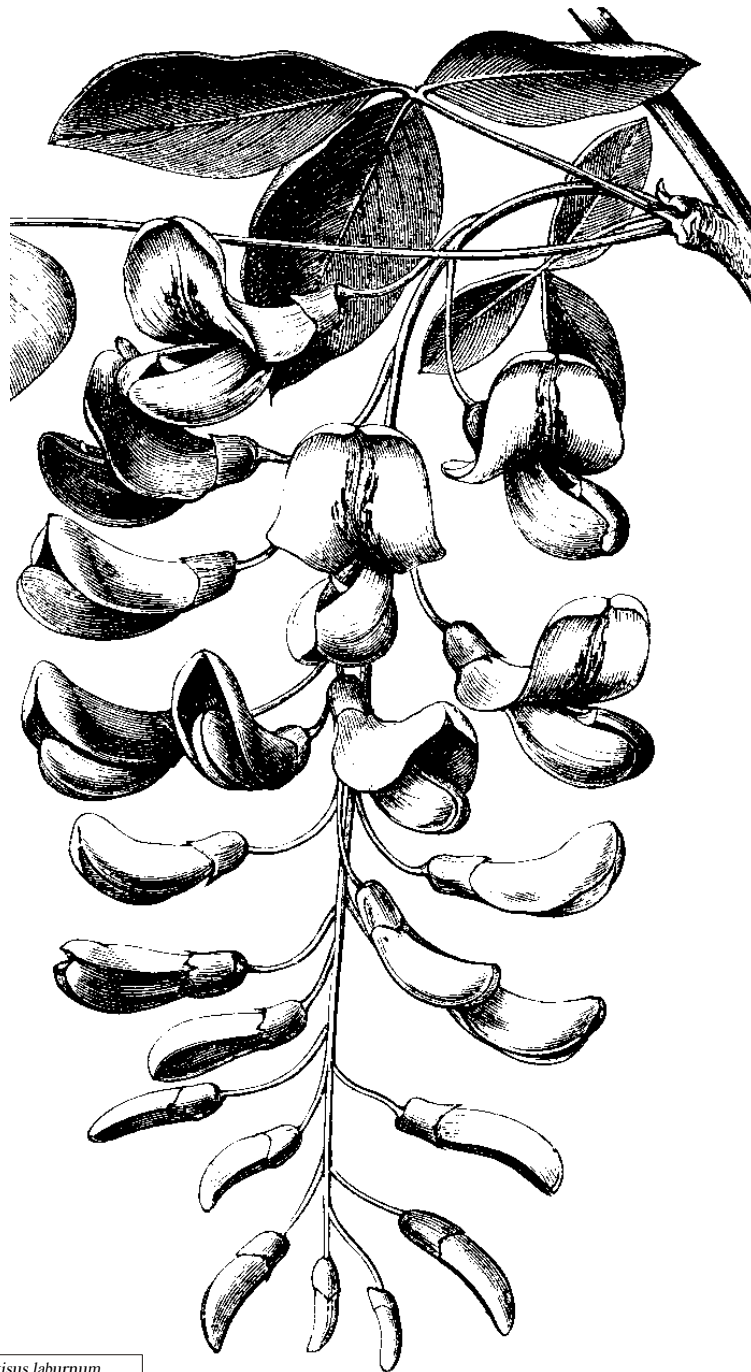
Cytisus laburnum after FAGUET — 1891
