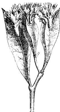
Statice thouini after FAGUET — 1892
