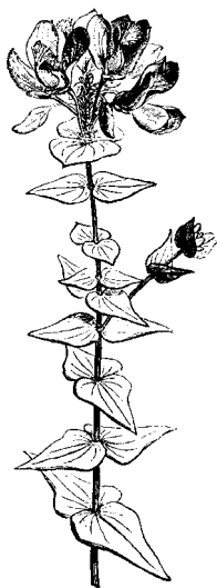
Polygala oppositifolia after FAGUET — 1888
