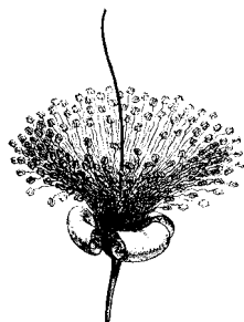
Acacia catechu after THIEBAULT — 1872
