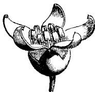
Bursera obtusifolia after FAGUET — 1878
