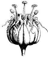
Leek — Allium ampeloprasum var porrum after FAGUET — 1888
