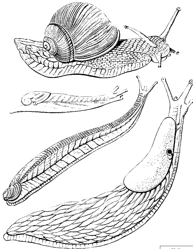
Helix pomatia & other Pulmonata
