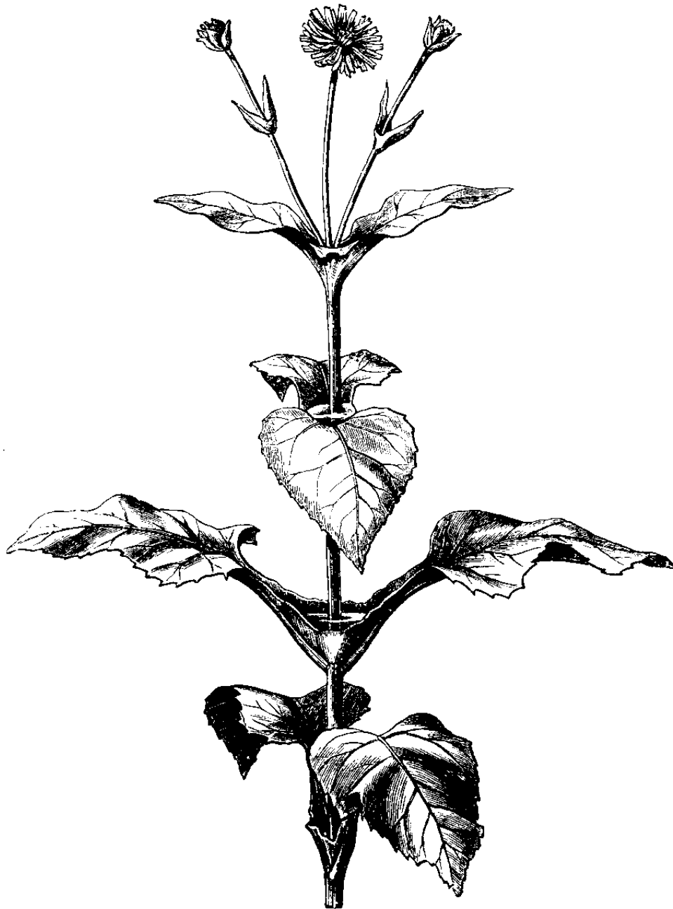
Silphium perfoliatum after THIEBAULT — 1888
