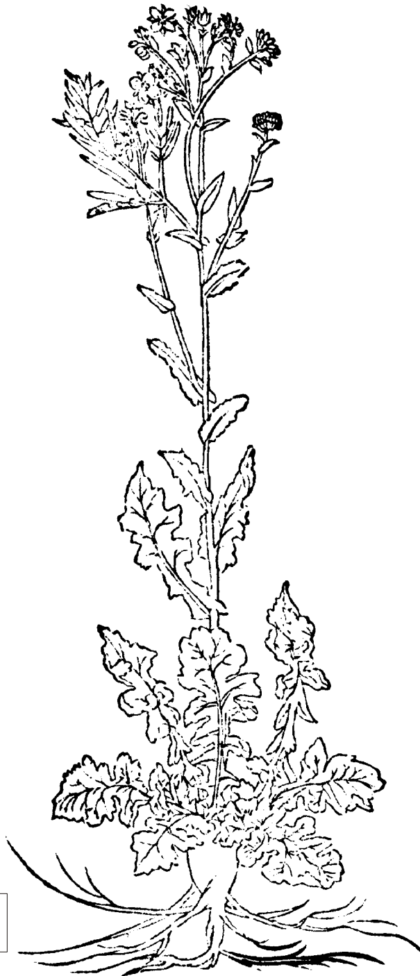
Napus Bunias sylvestris from FUCHS — 1545
