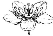
Agrimonia eupatoria after FAGUET — 1888
