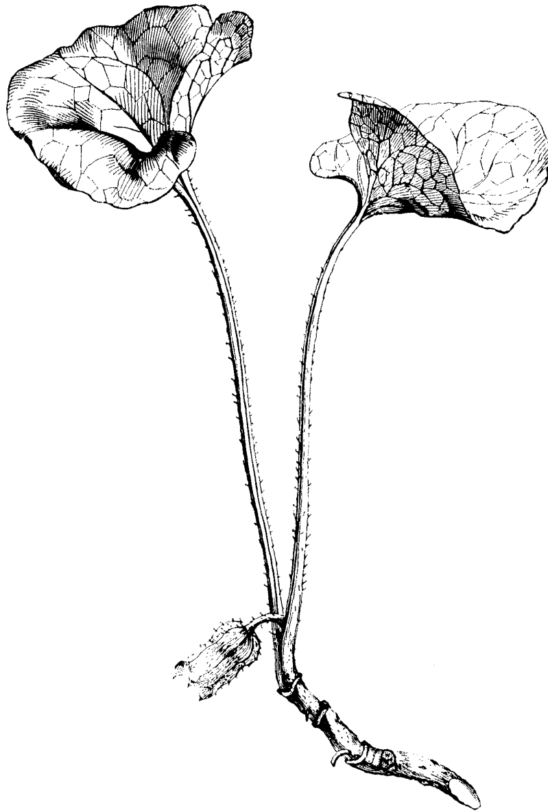
Asarum europaeum after FAGUET — 1888
