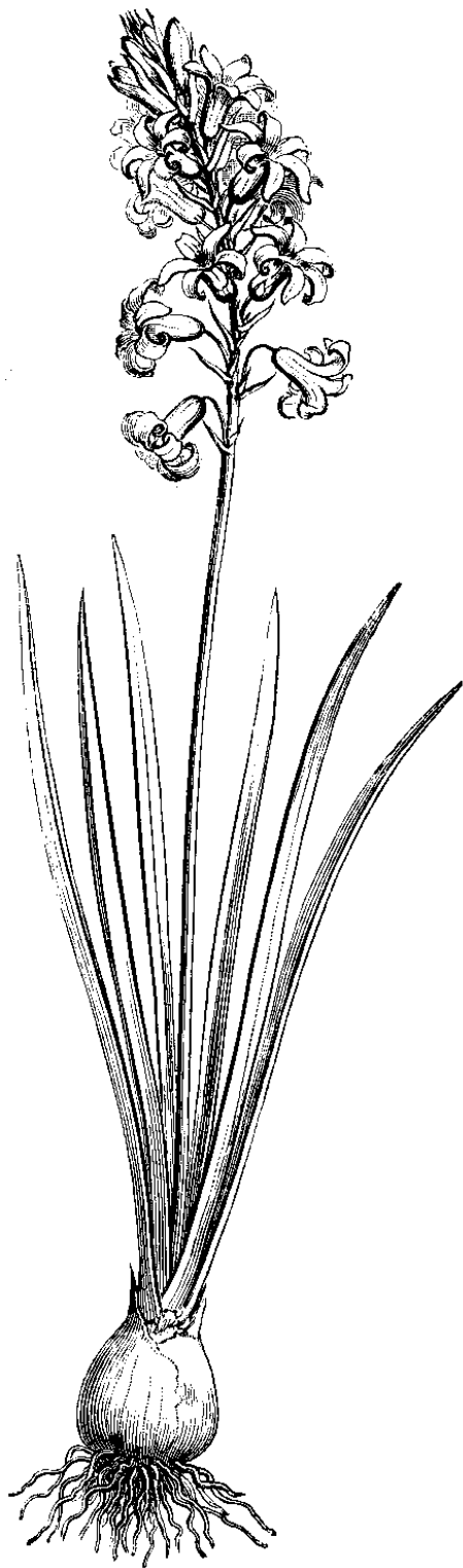
Scilla non scripta after FAGUET — 1888
