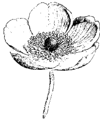
Anemone alba after FAGUET - 1888
