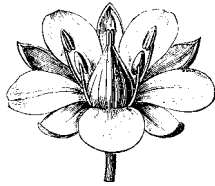
Telephium imperati after FAGUET — 1888
