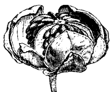
Elatine paludosa after FAGUET — 1888
