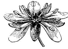
Balanites aegyptica after FAGUET — 1875
