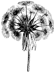
Lactuca virosa [seed head] after FAGUET — 1880
