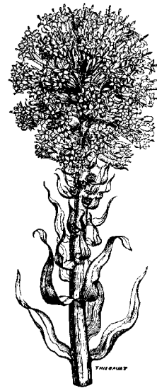
Petasites officinalis after THIEBAULT — 1888
