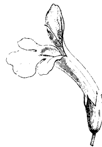
Betony - Betonica officinalis , Stachys officinalis after FAGUET — 1888
