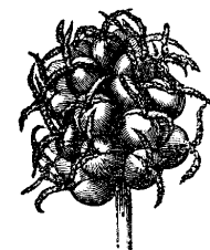
Morus alba after FAGUET — 1880
