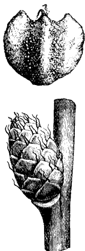
Myrica gale after FAGUET — 1880
