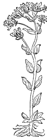
Centaureum minus from FUCHS — 1545
