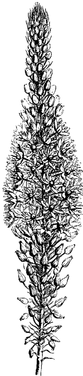
Urginea maritima after FAGUET — 1888
