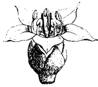
Dodder — Cuscuta epithymum after FAGUET — 1888
