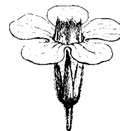
Alkanet [Bugloss] - Anchusa italica after FAGUET — 1888
