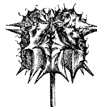
Tribulus terrestris after FAGUET — 1874
