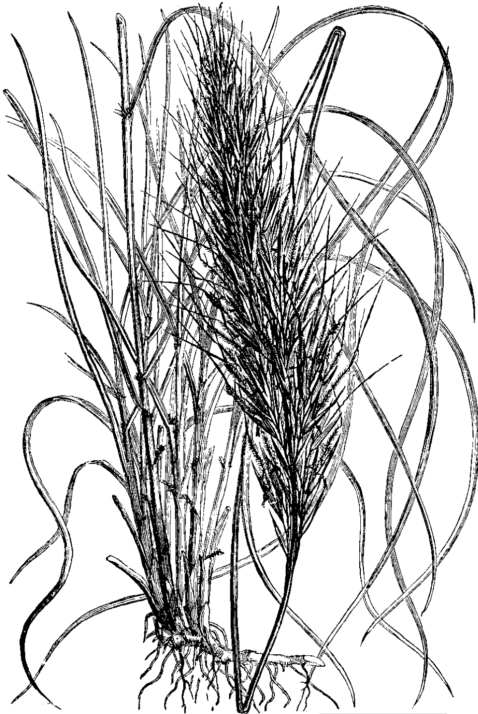
Stipa tenacissima after FAGUET — 1894
