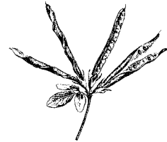
Lotus corniculatus after FAGUET — 1880
