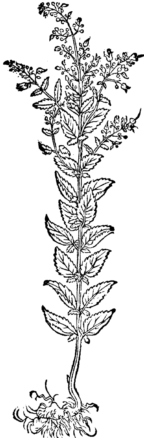
Galeopsis minor after FUCHS — 1545
