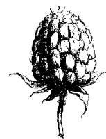
Rubus idaeus after FAGUET — 1888
