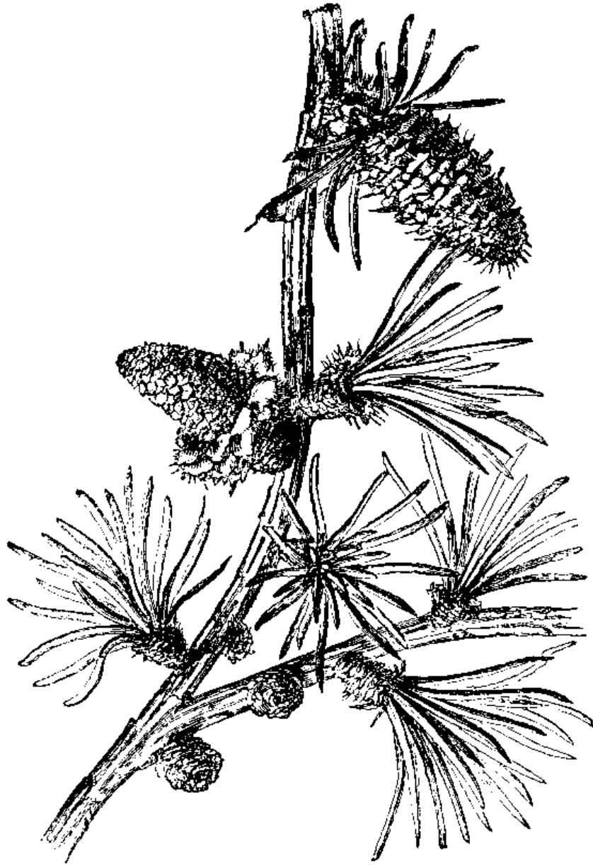
Pinus larix after FAGUET— 1888
