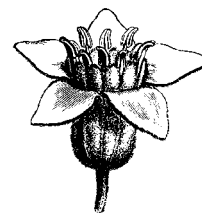
Aquilaria malaccensis after FAGUET — 1888
