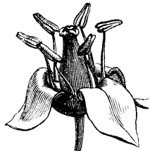
Bursera gummifolia after FAGUET — 1878
