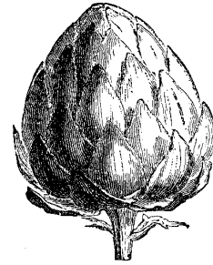
Carduus scolymus after FAGUET — 1880
