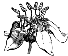
Bursera gummifolia after FAGUET — 1878
