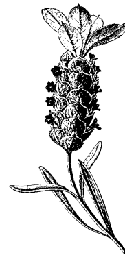
Lavandula stoechas after WINKLER — 1891
