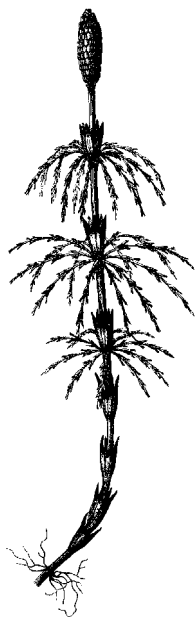
Equisetum sylvaticum after FAGUET — 1891
