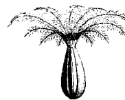
Valeriana officinalis after THIEBAULT — 1881
