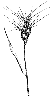
Triticum ovatum after FAGUET — 1894
