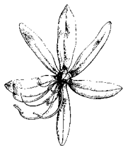
Asphodel Asphodelus luteus after FAGUET — 1888
