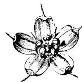
Paronychia serpyllifolia after FAGUET — 1888
