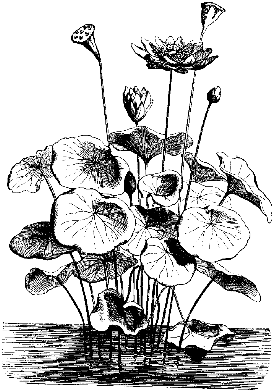
Nelumbo nucifera after FAGUET — 1888
