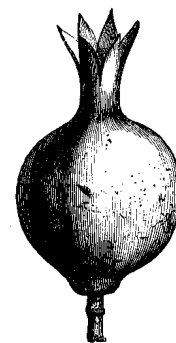
Punica granatum after FAGUET — 1880
