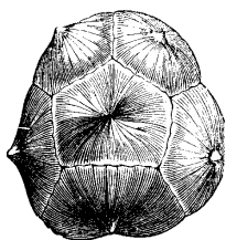
Cupressus sempervirens after FAGUET— 1888
