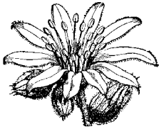
Sempervivum tectorum after FAGUET — 1888
