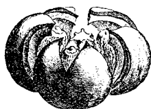
Euphorbia lathyris after FAGUET — 1878
