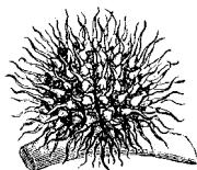
Sparganium ramosum (female inflorescence) after FAGUET — 1894
