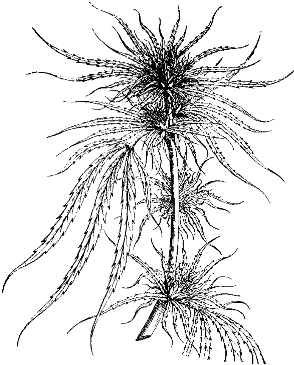
Cannabis sativa after FAGUET — 1880
