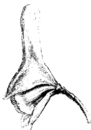
Aconitum lycoctonum after FAGUET — 1894
