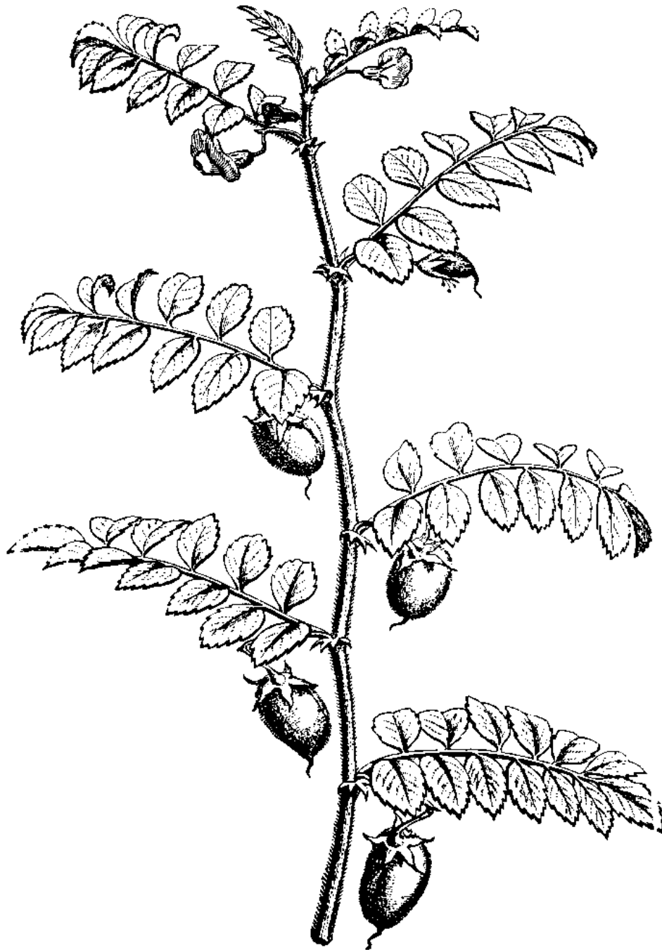
Cicer arietinum after FAGUET — 1888
