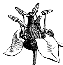
Bursera gummifera after FAGUET— 1888
