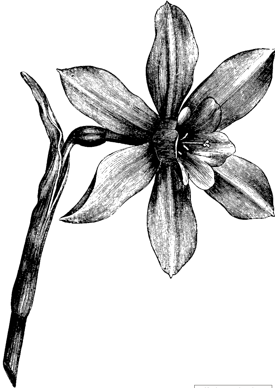
Narcissus pseudonarcissus after FAGUET — 1891
