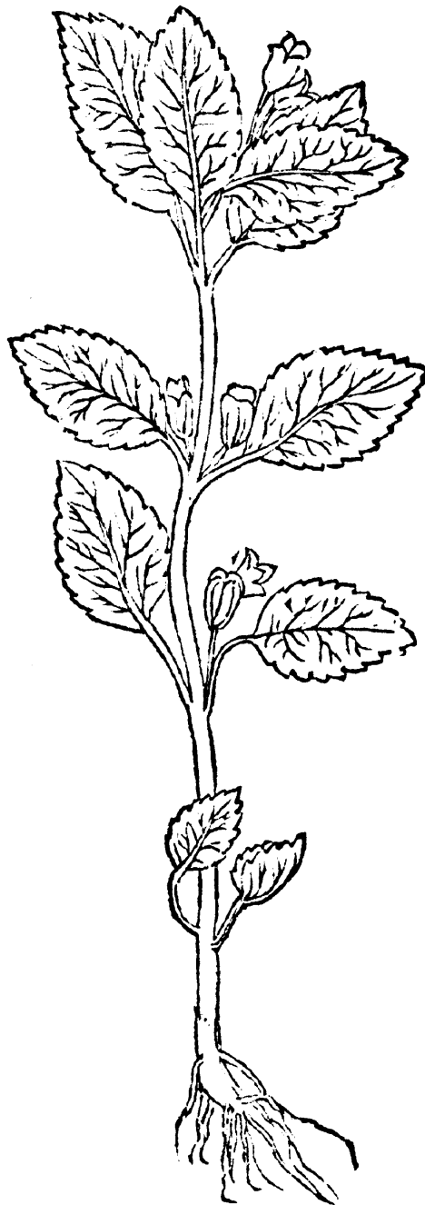
Melissophyllum uerum from FUCHS — 1545
