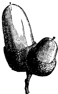
Quercus robur after FAGUET — 1880
