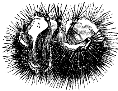
Castanea vulgaris — Chestnut after FAGUET — 1880
