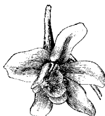
Delphinium peregrinum after FAGUET — 1894
