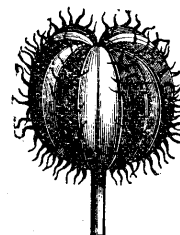
Ricinis communis after FAGUET — 1888
