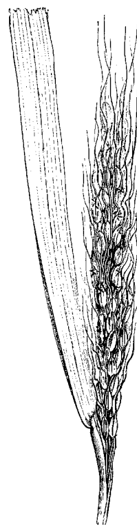
Oryza sativa after FAGUET — 1892
