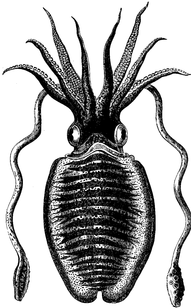
Sepia officinalis after OWEN — 1909
