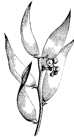
Ruscus racemosus after FAGUET — 1888
